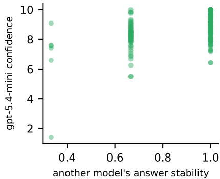
confidence vs cross-model stability r = +0.410
