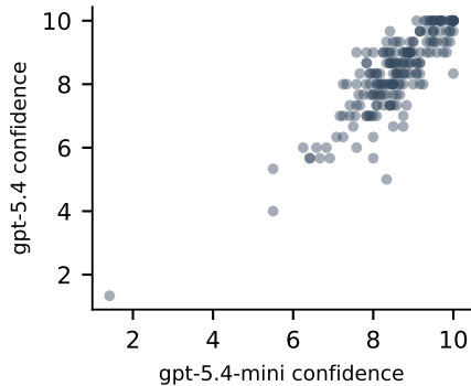
cross-model confidence r = 0.853
