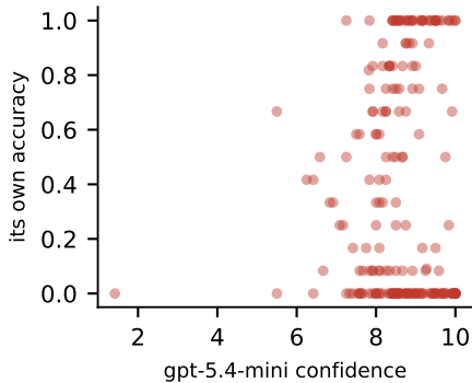
confidence vs own correctness r = +0.075
