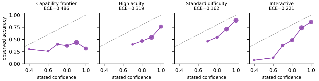
Fig. 6. Reliability diagrams, gpt-5.4-mini; marker area is proportional to bin occupancy and the dashed line is perfect calibration. At the capability frontier the curve is essentially flat—observed accuracy is unrelated to stated confidence over its whole range—whereas the interactive curve is monotone. Expected calibration error is reported above each panel, and moves in the same direction as discrimination without being equivalent to it.
