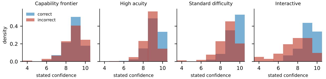
Fig. 5. Distribution of stated confidence for correct (blue) and incorrect (red) episodes, gpt-5.4-mini. At the capability frontier the two distributions are superimposed; separation appears at standard difficulty and is widest under interactive consultation.
