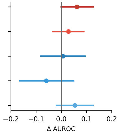
discrimination restored
