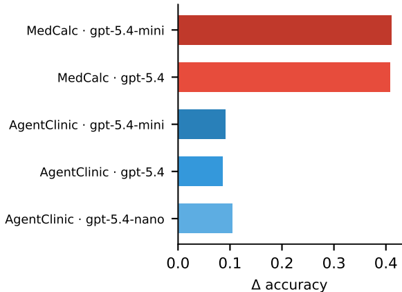
accuracy restored
