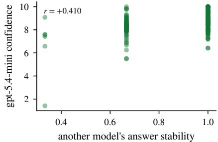
confidence vs peer stability
