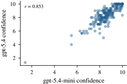
cross-model confidence
