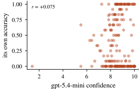
confidence vs own correctness
