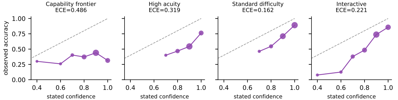
Fig. 3. Reliability diagrams, gpt-5.4-mini; marker area is proportional to bin occupancy and the dashed line is perfect calibration. At the capability frontier the curve is essentially flat—observed accuracy is unrelated to stated confidence over its whole range—whereas the interactive curve is monotone. Expected calibration error is reported above each panel, and moves in the same direction as discrimination without being equivalent to it.
