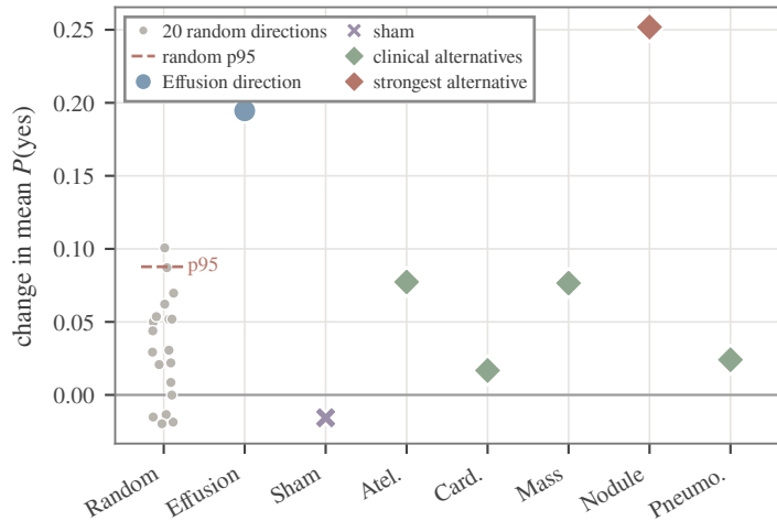
(a) locked dose \alpha = +0.25 , 400 new patients
