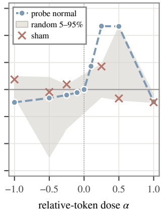
(c) Qwen2.5-VL-7B, Effusion
