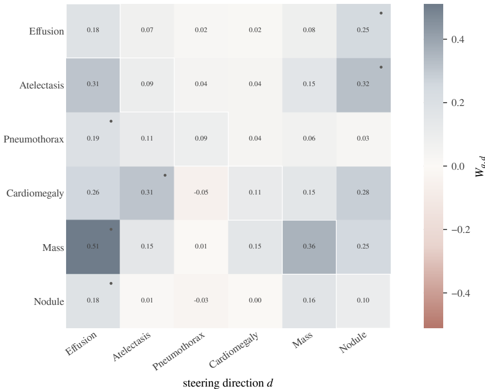
Qwen2.5-VL-7B, 400 patients, \alpha = +0.25 ; dot = column-wise strongest direction (all off-diagonal)
