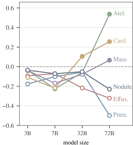
(a) Qwen2.5-VL on NIH ownership appears at 32B and 72B
