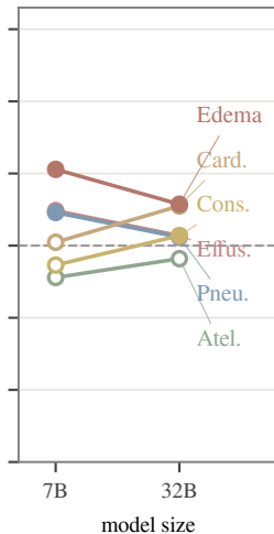
(c) Lingshu on CheXpert five of six owned at 32B
