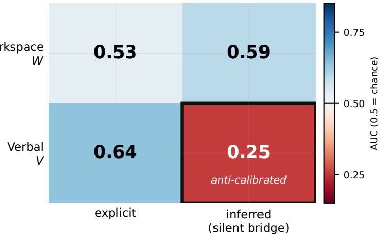
AUC by regime × channel (Qwen-3B)
