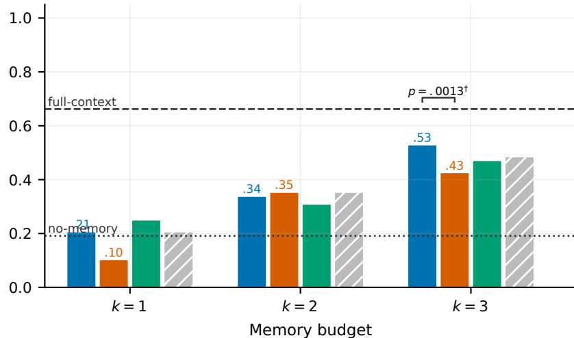
(b) Qwen-7B, Decoupled, 68 episodes
