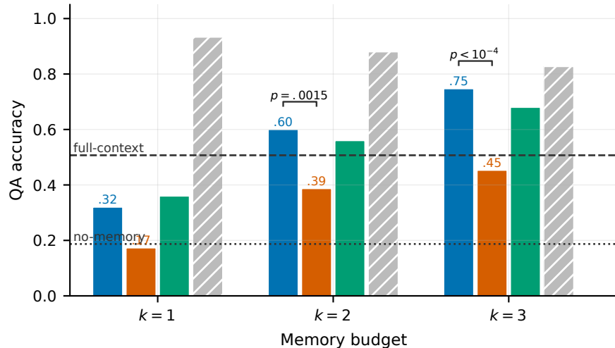
(a) Qwen-0.5B, Evoked, 75 episodes
