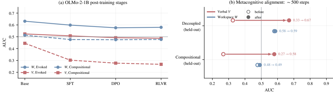
Figure 6: Post-training changes the verbal channel, not the workspace channel, and the verbal channel is repairable. (a) OLMo-2-1B released post-training stages: the workspace channel ( W , blue) never improves from base, on either benchmark, while the verbal channel ( V , rose) stays at chance (Evoked) or far below it (Compositional). (b) Metacognitive alignment: \sim 500 self-distillation steps move the verbal channel (arrows) from below-chance to well-calibrated on fully held-out benchmarks while leaving the workspace channel in place (open circle = before, filled = after).
