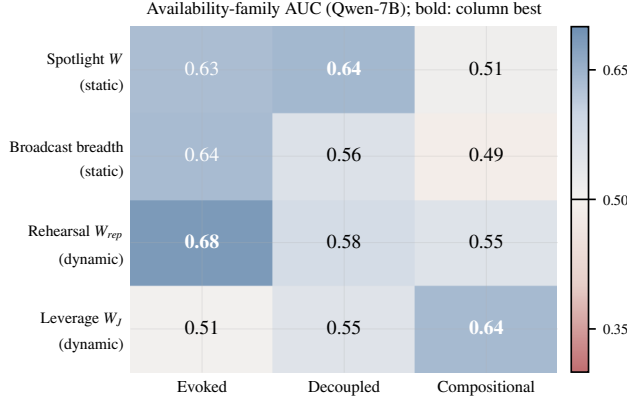
Figure 7: The availability-family double dissociation as a matrix (Qwen-7B): decode-based members (rows 1–3) own the Evoked regime; the utility-gradient member (row 4) is the only readout with a significant paired gain over the static readout on the Compositional benchmark (Table 5); the conditional-likelihood baseline’s nominal edge there does not reach significance (App. J).
