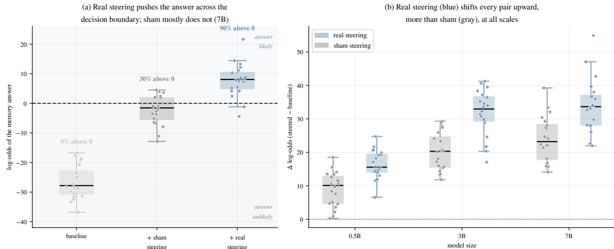
Figure 5: The workspace direction is causally load-bearing. Steering the residual stream along the stored bridge’s input-side direction, while the model answers from memory, versus norm-matched sham directions built from unrelated held-out bridges (20 disjoint pairs). (a) At 7B the memory answer starts far below the decision boundary (baseline log-odds median -27.8 ; 0% of pairs above 0); real steering moves 90% of pairs above it, sham only 30%. (b) The per-pair shift is positive for every pair at all three scales and larger for real than sham throughout. The direction the readout scores is the direction that decides the answer.
