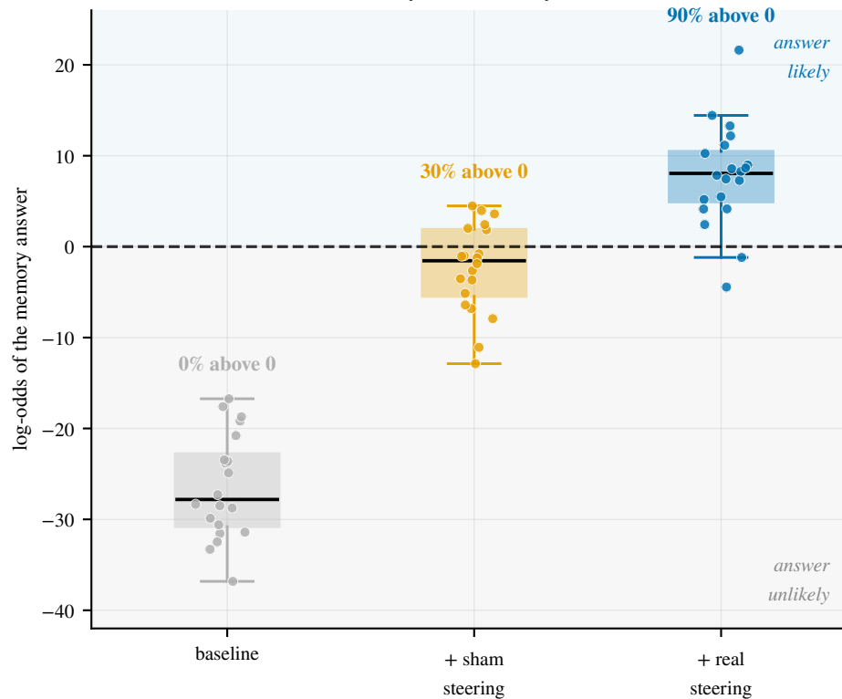
(a) Real steering pushes the answer across the decision boundary; sham mostly does not (7B)
