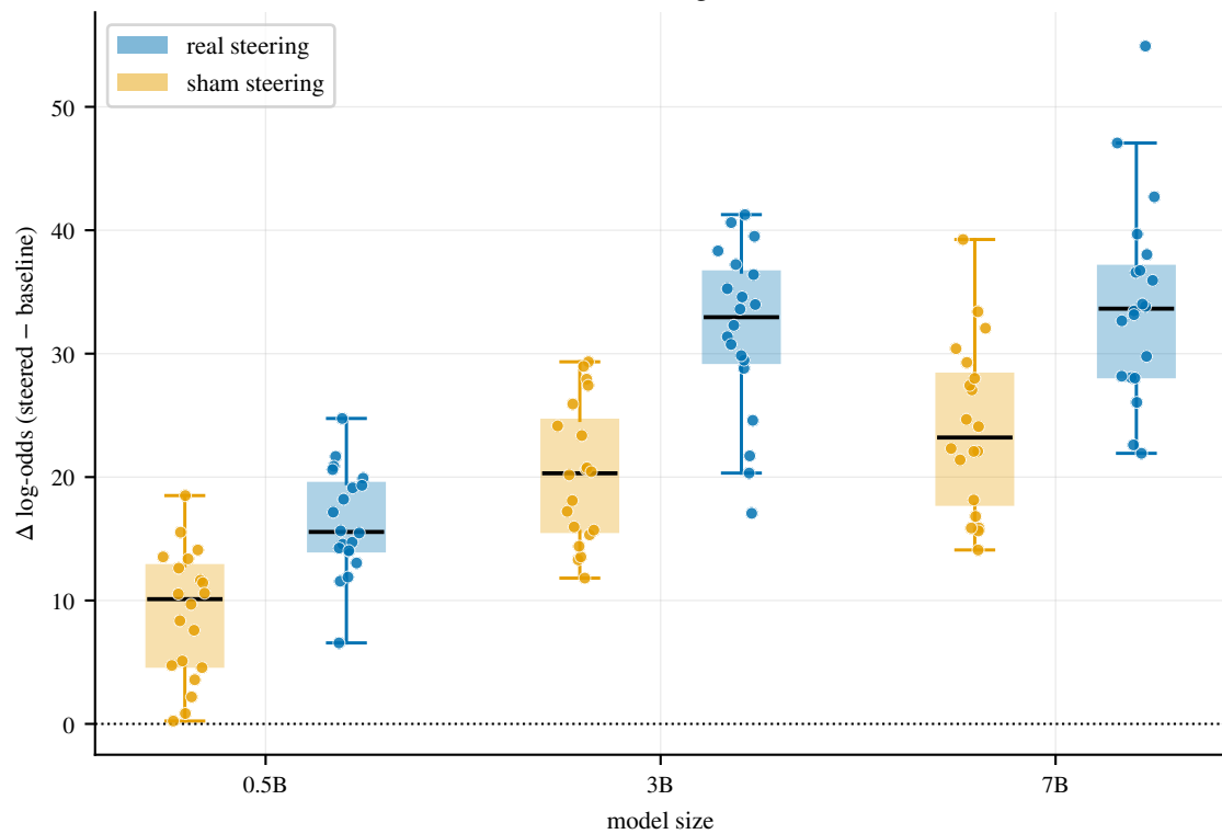
(b) Real steering (blue) shifts every pair upward, more than sham (orange), at all scales
