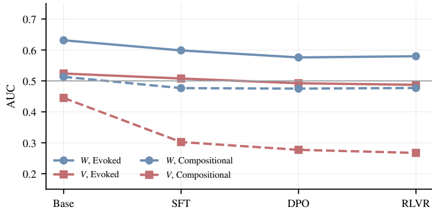
(a) OLMo-2-1B post-training stages
