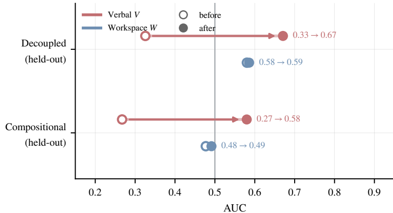
(b) Metacognitive alignment: \sim 500 steps
