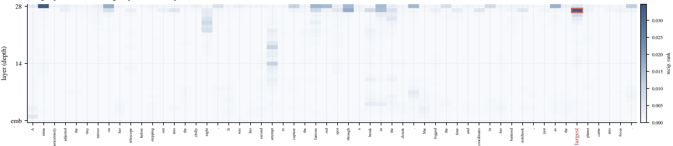
bridge “ganges” (``the sacred river" → India)
