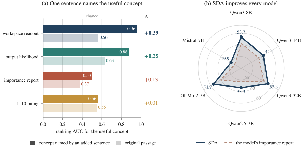
Figure 1: Naming the useful concept raises AUC far more for the workspace readout and output likelihood than for the importance report and 1–10 importance rating; Self-Distilled Admission (SDA) distills these two rankings into admission decisions. (a) Six-model mean pooled AUC on the standard pool: original passage (pale) or with one added sentence naming the useful concept (solid); dashed line: chance. (b) Answer accuracy (%) at two stored concepts on the statedness-balanced pool: SDA (solid, three-seed mean) against each model’s report (dashed); mean gain 9.8 points.
