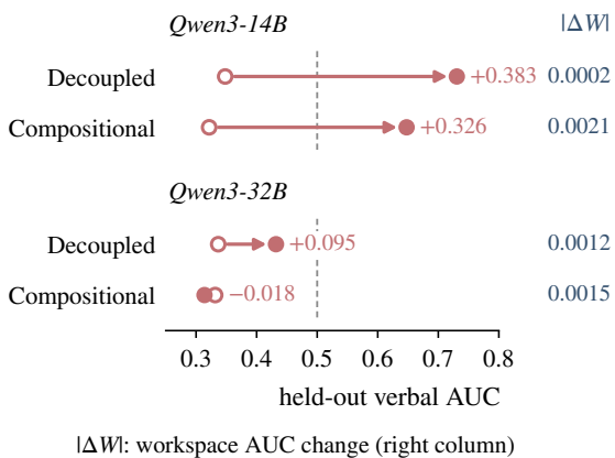
(b) Qwen3-14B and 32B, one seed each
