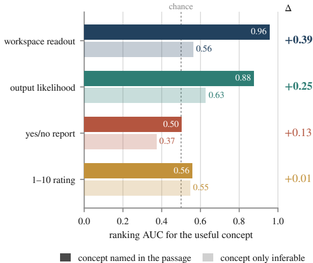
(a) One sentence names the useful concept
