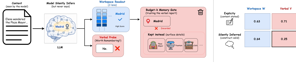
Figure 1: Left: the write-gating problem. Reading “Elena wandered the Plaza Mayor. . .”, the model silently infers madrid , and the inference is visible in a J-lens-style workspace readout of its residual stream; asked whether madrid is worth remembering, it confidently says no. A budget- k memory gate that trusts the verbal report discards exactly the item needed to answer “What language should Elena use?”. Right: AUC of each channel at identifying truly load-bearing items (Qwen-3B shown; same qualitative dissociation at 3B–7B in all four families, with knife-edge small-scale cells noted in App. P; Table 1): the verbal report is good for explicit content but below chance for construct-valid silently inferred content (boxed cell; generator analysis in §5.1); the workspace readout is not.
