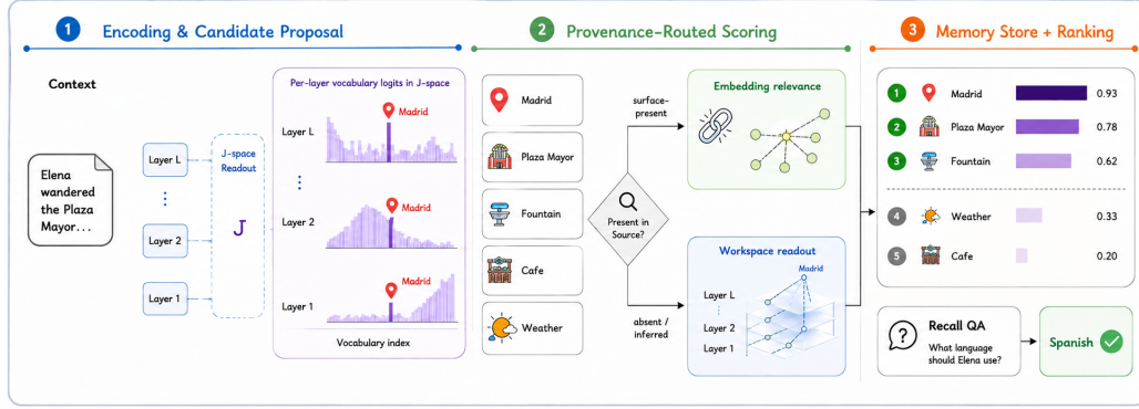
Figure 2: The PRG write gate, on the running example. Reading “Elena wandered the Plaza Mayor...”, the model silently infers the bridge Madrid , a concept that never appears in the text. A J-lens “J-space” readout exposes each candidate’s per-layer vocabulary logits across the residual stream; the workspace score is the peak reciprocal rank of the candidate’s token over layers (Eq. 5). Each candidate proposed by the host memory system is then routed by the provenance test \rho (here a substring check against the source context): surface-present items ( Plaza Mayor , Fountain , ...) are scored by embedding relevance, while absent, inferred items ( Madrid ) are scored by the workspace readout, the channel that tracks their utility most reliably in our experiments. Percentile-rank calibration places both routes on a common scale, and budget- k admission keeps the top-ranked items (dashed cutoff): the inferred Madrid is admitted rather than discarded, so the downstream recall question “What language should Elena use?” is answered correctly ( Spanish ). The gate adds no training and no model calls beyond the encoding pass.
