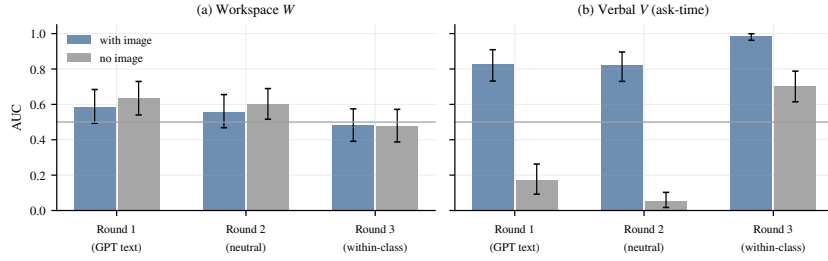
Figure 12: Multimodal double ablation (Qwen2-VL-2B, landmark photos): the end-of-encoding word-level workspace never distinguishes the pictured city within-class (a), while ask-time verbal probing reads the image nearly perfectly and collapses without it (b).
