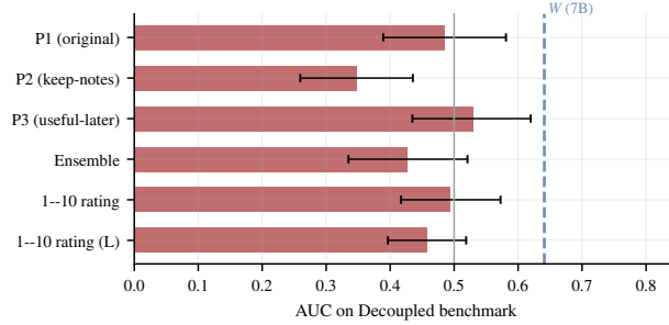
Figure 13: No verbal variant recovers sparse-cue construct-valid inferred content: three importance-probe paraphrases, their ensemble, and the canonical 1–10 rating (both Decoupled sizes) all sit at or below chance, against the workspace reference (dashed).
