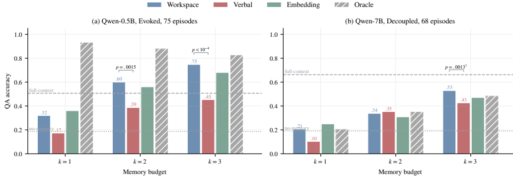
Figure 6: Budget-limited recall QA. Left: 0.5B on the Evoked benchmark, where workspace gating beats verbal gating ( k=2 : +20/-4 , p=0.0015 ; k=3 : +24/-2 , p<10^{-4} ), which sits at the no-memory floor. Right: 7B on the construct-valid Decoupled benchmark (64-token answers), where workspace gating matches the label oracle and beats verbal gating ( k=3 , \dagger : +26/-7 , p=0.0013 , computed on the 120-episode scaled benchmark). The two panels are the two regimes’ primary cells; the full grid, which also contains null and reversed cells at these n ’s, and all McNemar tests are in App. C.
