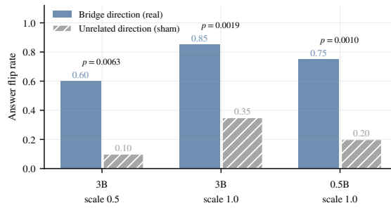
Figure 11: Causal check: steering along the stored bridge’s input-side direction (real) flips memory-based answers far more often than an unrelated direction (sham); disjoint episode pairs, exact McNemar p above each pair of bars.
