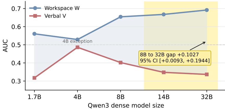
Figure 5: Corrected Qwen3 Decoupled scale sweep. Yellow shading marks the newly added 14B/32B boundary region; the original figures elsewhere in the paper are retained.
