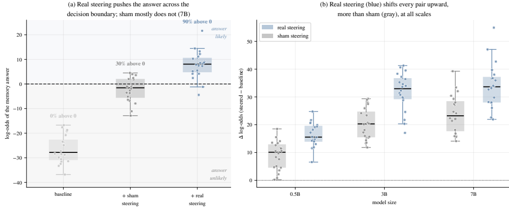
Figure 9: The workspace direction is causally load-bearing. Steering the residual stream along the stored bridge’s input-side direction, while the model answers from memory, versus norm-matched sham directions built from unrelated held-out bridges (20 disjoint pairs). (a) At 7B the memory answer starts far below the decision boundary (baseline log-odds median -27.8 ; 0% of pairs above 0); real steering moves 90% of pairs above it, sham only 30%. (b) The per-pair shift is positive for every pair at all three scales and larger for real than sham throughout. The direction the readout scores is the direction that decides the answer.
