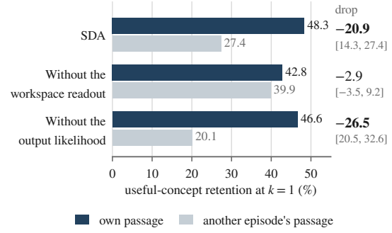
Figure 4: Replaced-passage test on the standard Fresh-2 pool, Qwen3-8B, 363 episodes. Retention is the percentage of episodes whose single stored concept is useful, with the episode’s own passage (solid) or another episode’s passage (pale); candidates, labels and question stay fixed. SDA and the students of teachers with one signal removed average three seeds. Drops give paired 95% intervals from 4,000 episode-bootstrap draws; Table 30 adds the untrained readouts.
