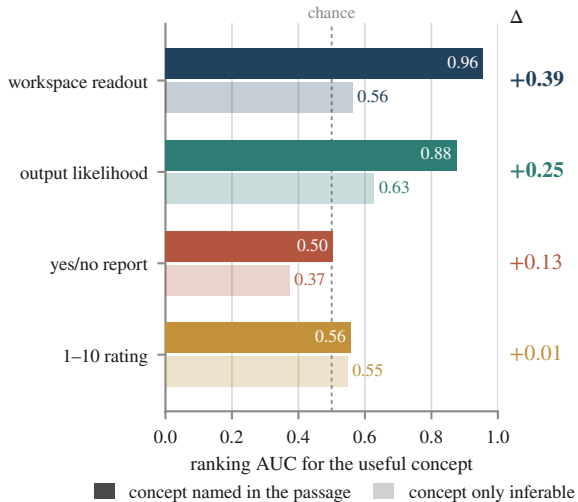
(a) One sentence names the useful concept
