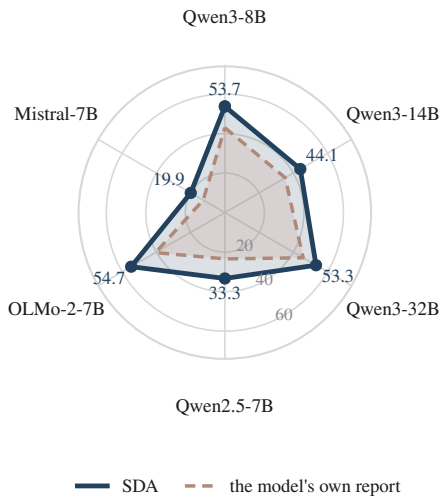
(b) SDA improves every model
