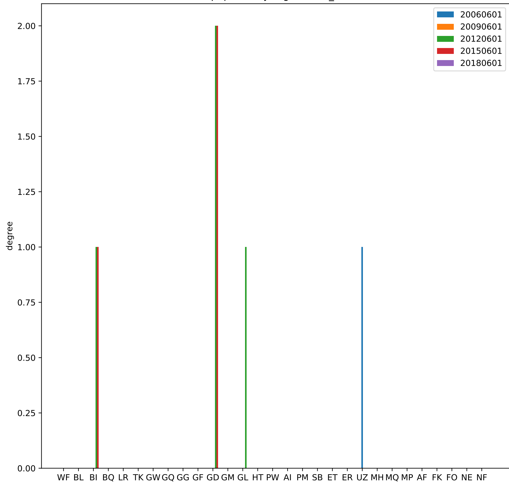
p2pCountryDegreeInter_0
