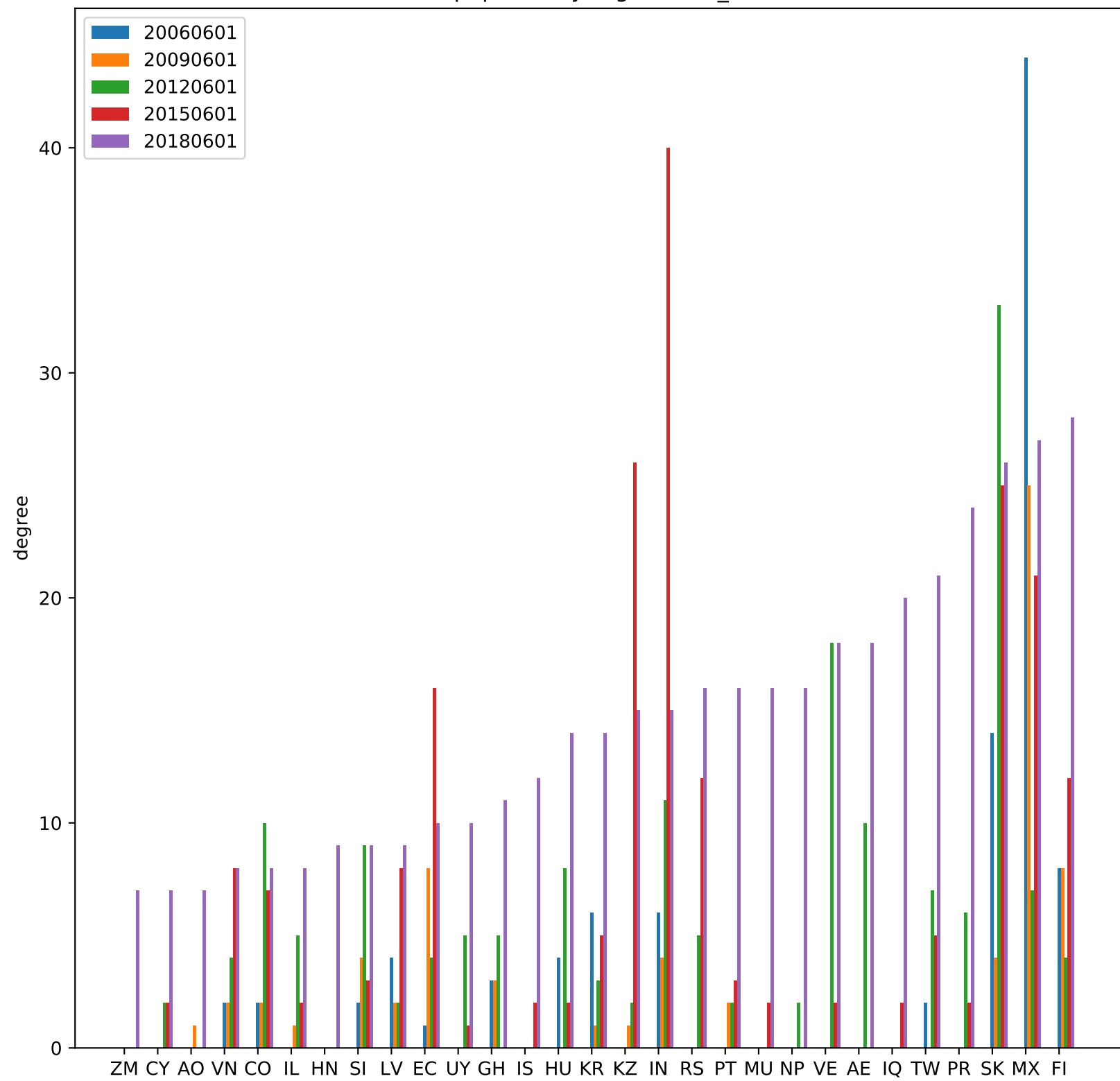
p2pCountryDegreeIntra_6
