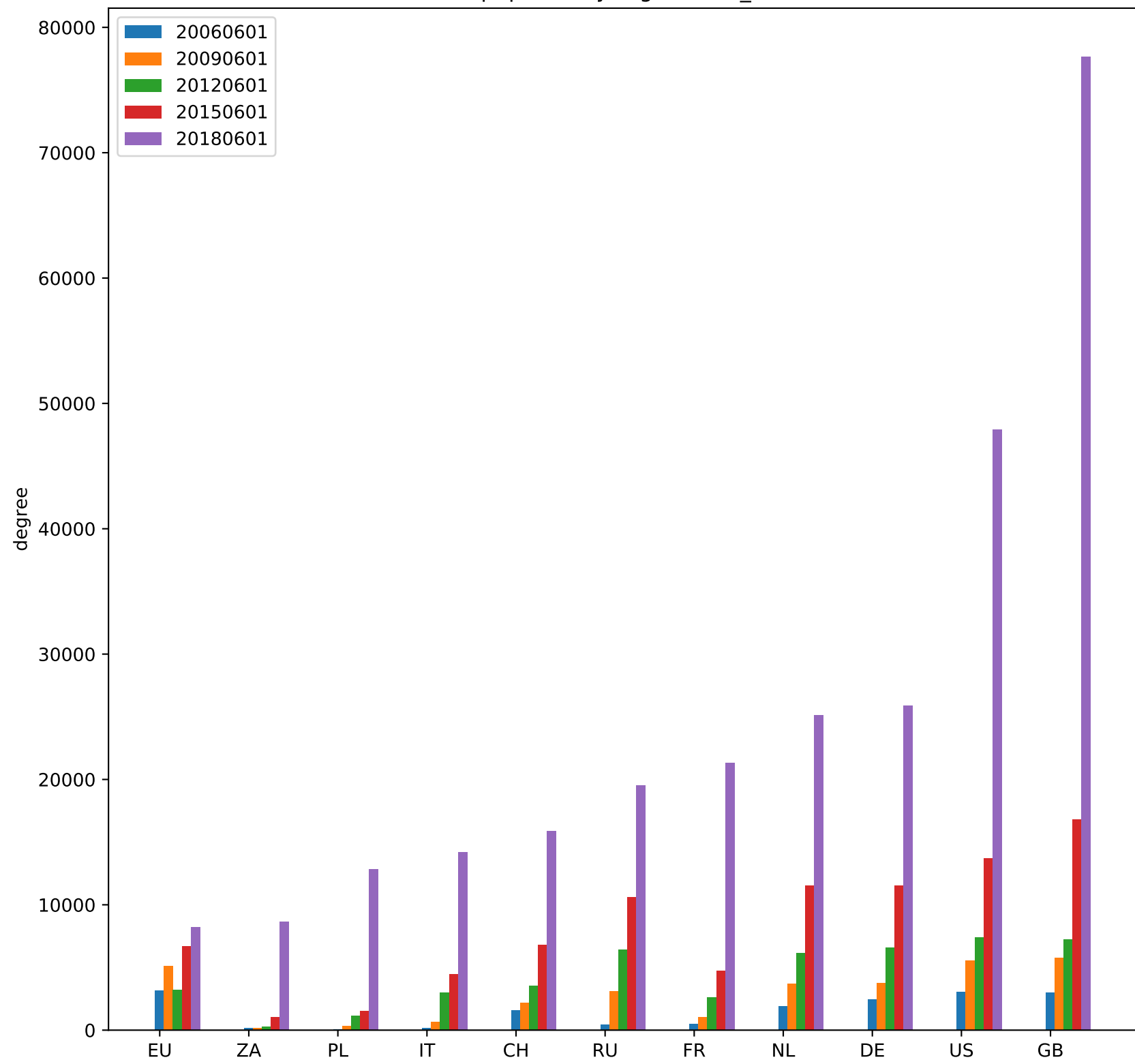
p2pCountryDegreeInter_8
