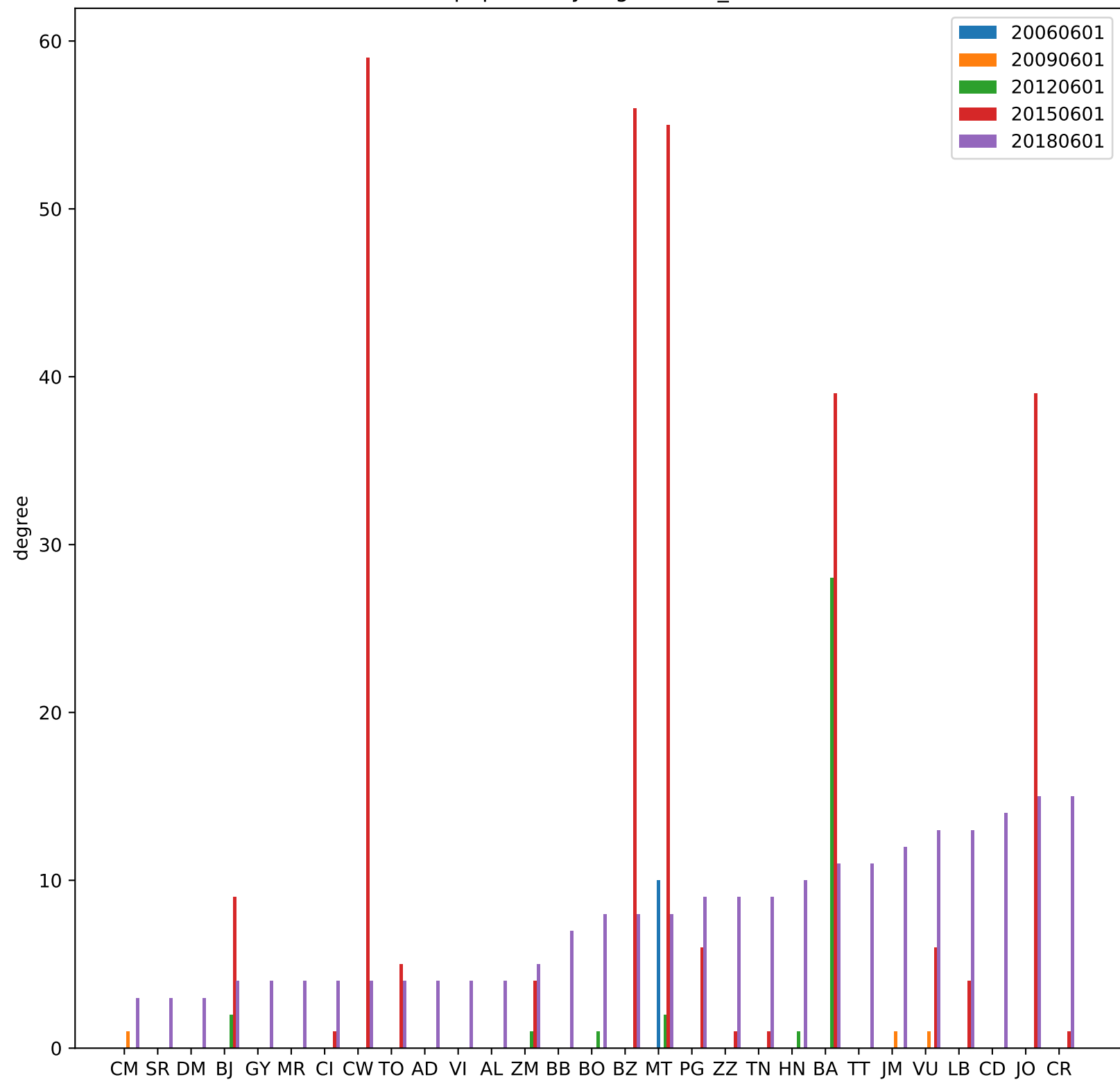
p2pCountryDegreeInter_3
