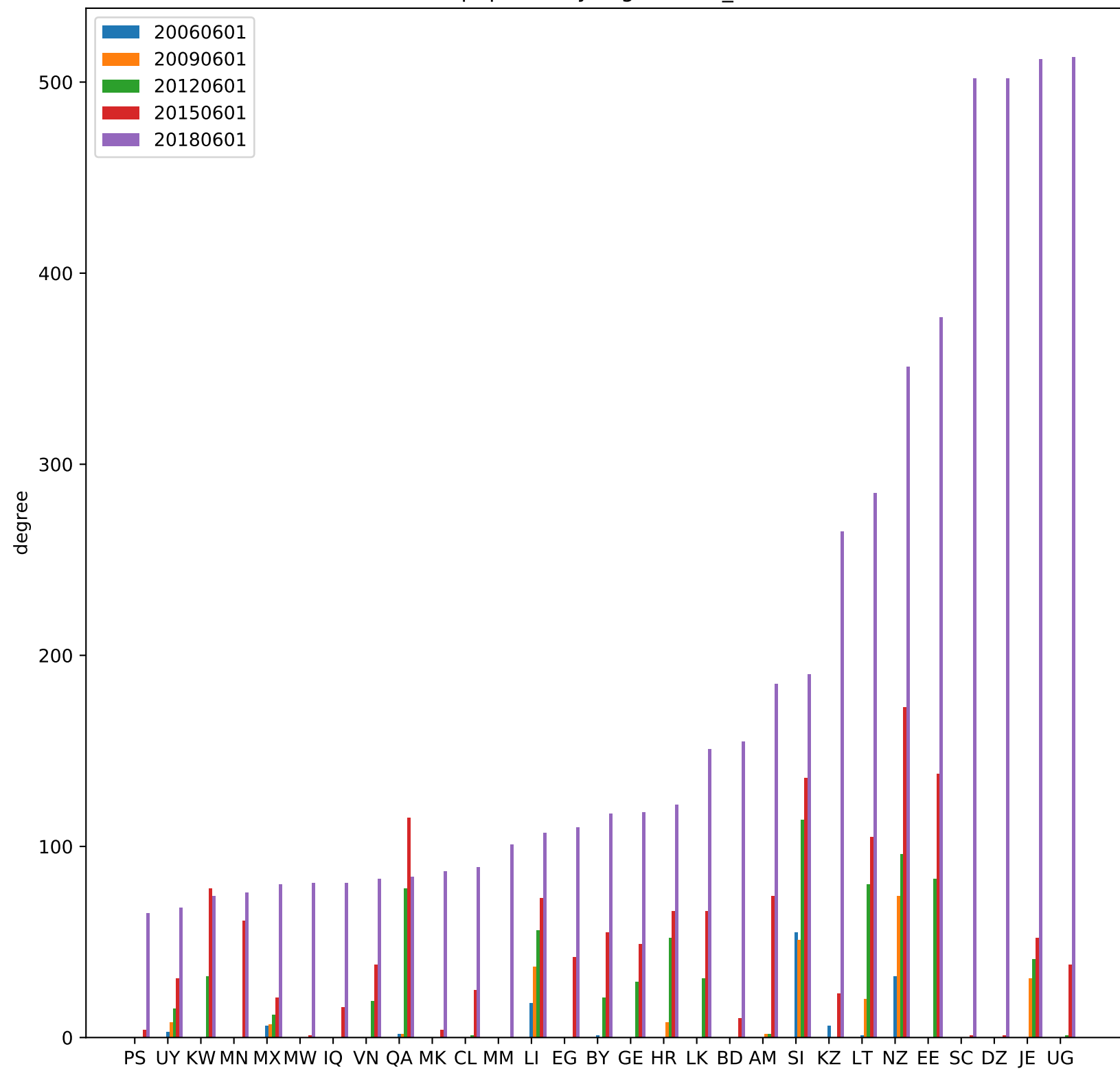
p2pCountryDegreeInter_5
