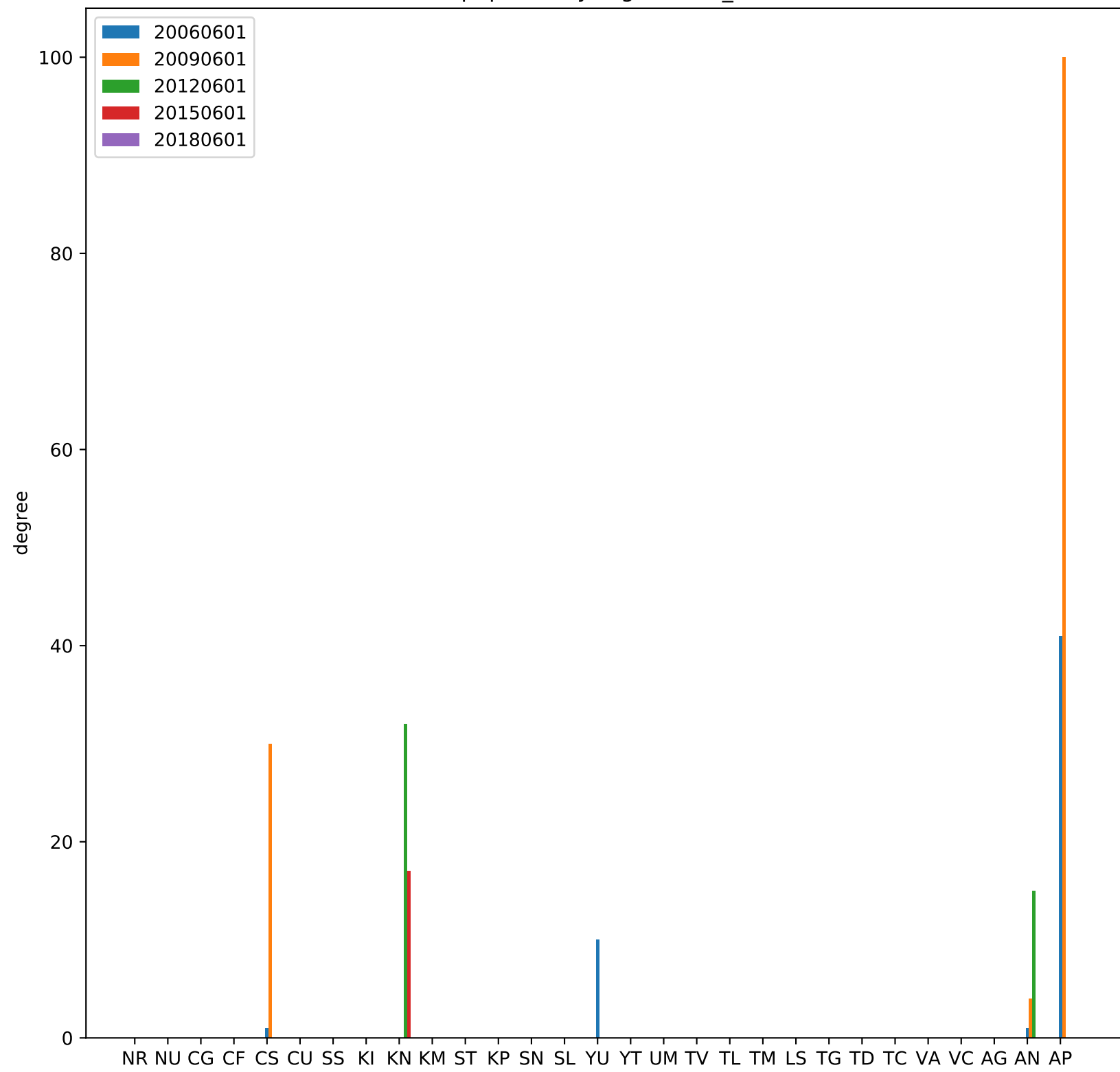
p2pCountryDegreeInter_1
