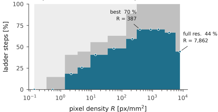
(b) pixels — same decision, input downscaled
