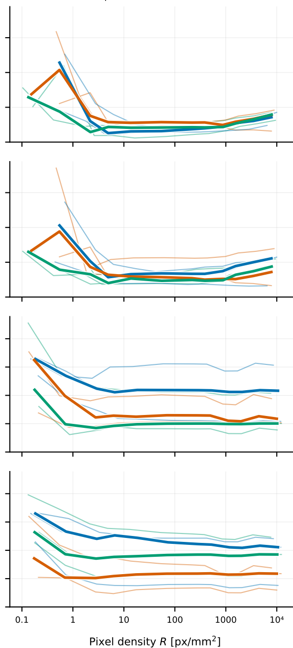
Shape reconstruction error
