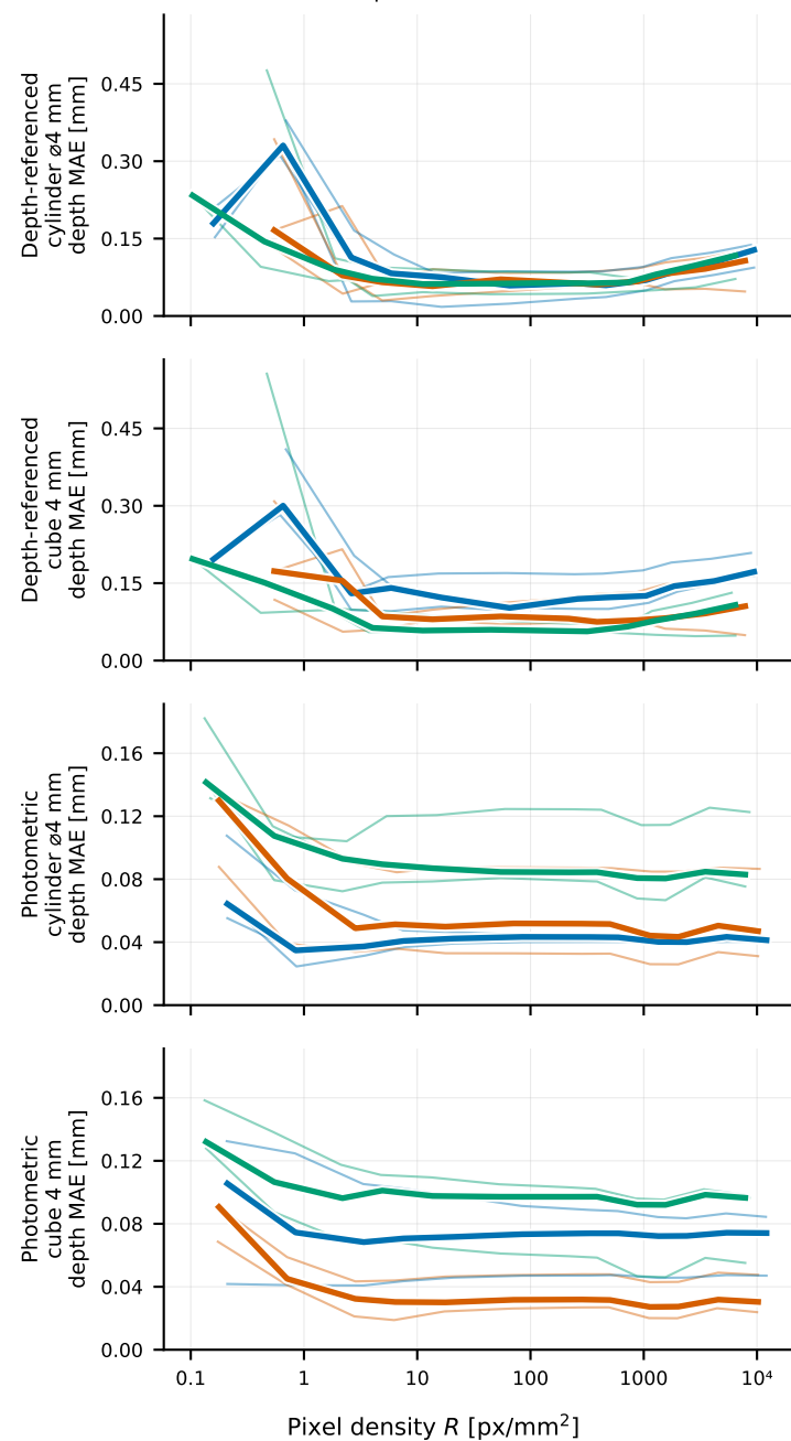
Shape reconstruction error
