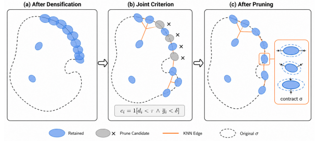
Figure 4: Geometry-aware Pruning (GAP). After gradient-driven densification, Gaussians cluster around high-contrast boundaries. GAP flags a Gaussian as a redundancy candidate only when it is both locally crowded ( d_i < \tau ) and recently inactive ( \bar{g}_i < \delta ), so that capacity is reclaimed from saturated boundaries without removing Gaussians that are still learning structure.
