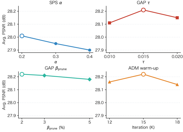
Figure 12: Hyperparameter sensitivity analysis in the 3-view setting. The four subplots correspond to the SPS sampling mixture coefficient \alpha , the GAP proximity threshold \tau , the maximum pruning ratio \beta_{\text{prune}} , and the ADM warm-up start iteration. The available results support a concentrated operating point rather than broad parameter insensitivity.
