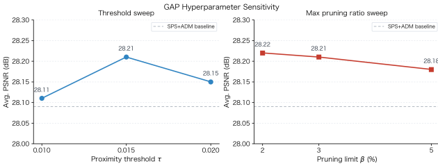
Figure 13: Local hyperparameter sweep for GAP. The left panel studies the proximity threshold \tau , and the right panel studies the maximum pruning ratio \beta_{\text{prune}} . The sweep suggests that the operating point used in the paper lies close to a local optimum in both curves.
