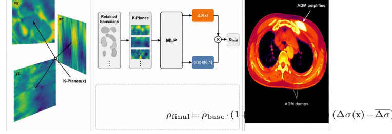
Figure 5: Adaptive Density Modulation (ADM). (a) Three orthogonal K-Planes feature maps (viridis) encode position-dependent spatial context for every Gaussian center. (b) The concatenated K-Planes feature is decoded by a lightweight dual-head MLP that predicts a density offset \Delta\sigma(\mathbf{x}) (orange) and a confidence gate g(\mathbf{x}) \in [0, 1] (slate); the modulated density combines them through \rho_{\text{final}} = \rho_{\text{base}} \cdot (1 + \tilde{o}) . (c) The resulting density difference map (inferno) shows that ADM amplifies density in regions where the attenuation support requires fine detail and damps modulation where evidence is uncertain.
