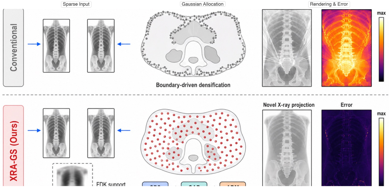
Figure 1: Comparison between a conventional sparse-view 3DGS workflow and XRA-GS . The top row summarizes the common error/gradient-driven densification pipeline in highly sparse CT, which tends to place newly spawned Gaussians near high-gradient anatomical boundaries. The bottom row shows our attenuation-aligned evolution pipeline, which uses coarse FDK support for path-anchored initialization, then reclaims redundant Gaussians with GAP and refines local density distributions with ADM. The figure emphasizes that our intervention targets the Gaussian evolution rule rather than the X-ray imaging equation itself.
