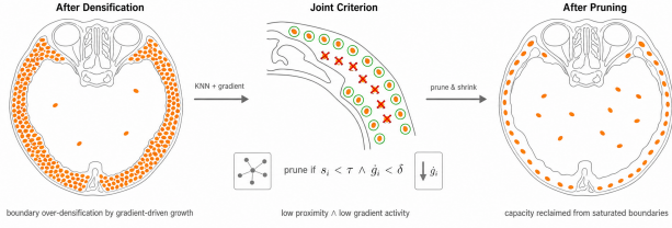
Figure 4: Geometry-aware Pruning (GAP).
