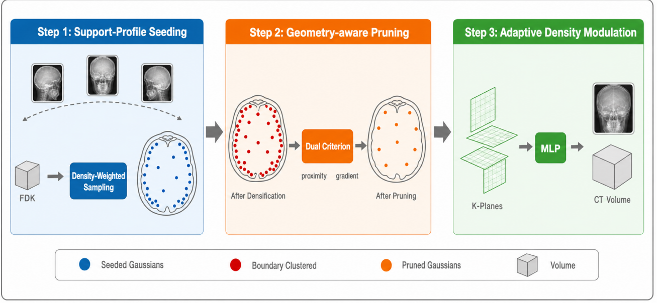
Figure 2: Overall framework of XRA-GS. Sparse X-ray projections together with a coarse FDK reconstruction enter a radiative Gaussian backbone whose adaptive density control is reorganized by SPS (seed), GAP (prune), and ADM (refine). The three modules act at initialization, inside the densification loop, and during later optimization, respectively, leaving inference unchanged.
