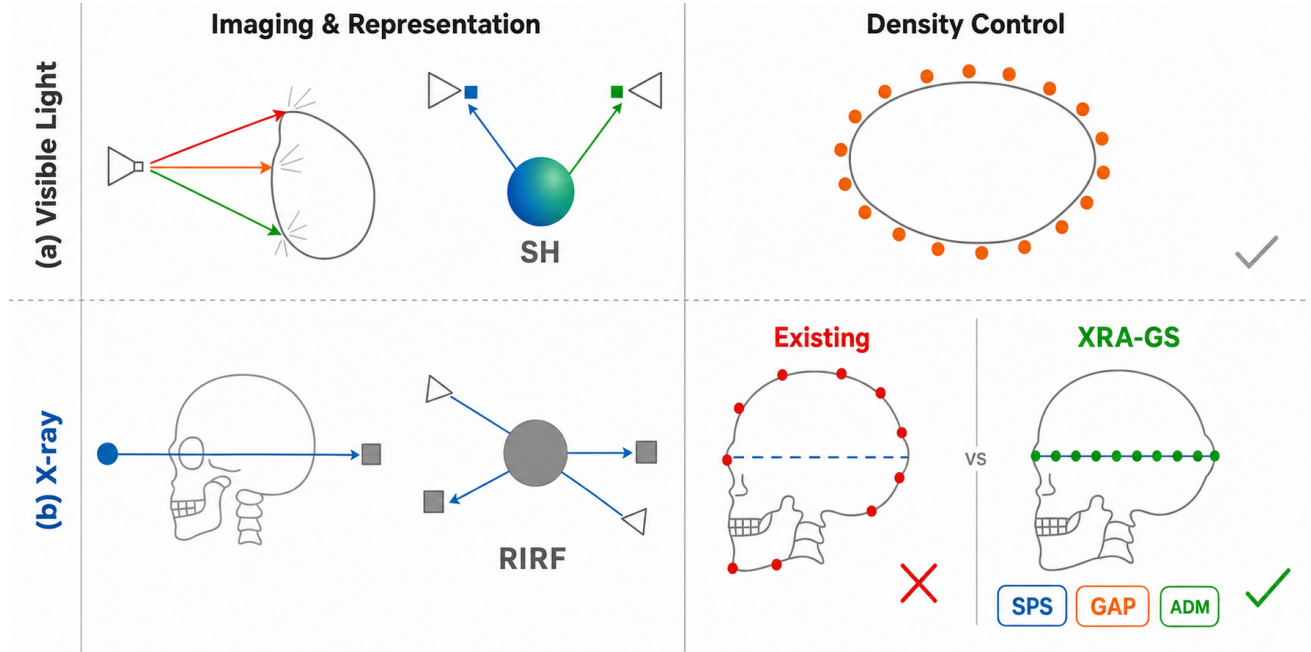
Figure 1: Visible-light vs. X-ray Gaussian rendering and the capacity gap they impose. (a) Visible-light \alpha -compositing concentrates capacity on visible surfaces, where front Gaussians occlude back ones. (b) X-ray line integrals weight every Gaussian along the ray equally, so naïve gradient-driven densification still clusters at attenuation boundaries; XRA-GS realigns the density control strategy through SPS, GAP, and ADM to anchor capacity along the path.
