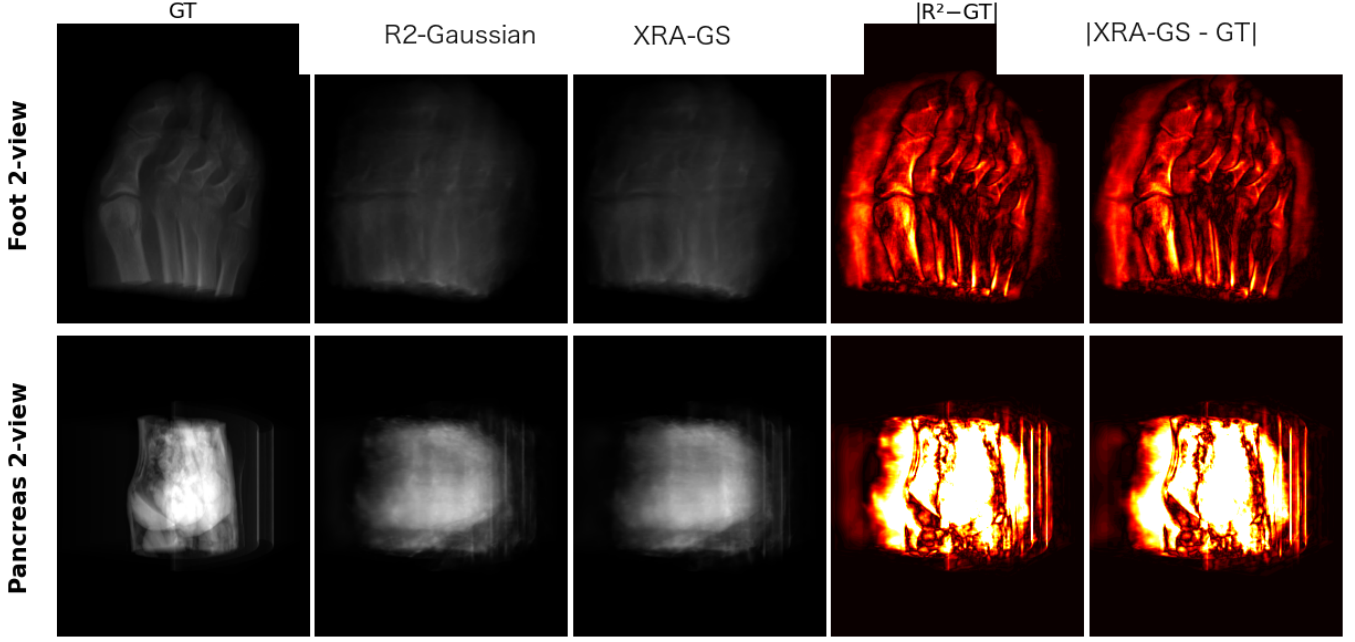
Figure 9: Representative failure cases. We show two more extreme under-determined cases, Foot 2-view and Pancreas 2-view , together with error maps of R 2 -Gaussian and XRA-GS relative to GT . When the input information is too limited or local structures are highly ambiguous, our method can still reduce error spread in some regions but cannot fully recover fine-grained detail.
