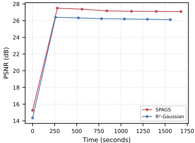
PSNR vs Wall-clock Time
