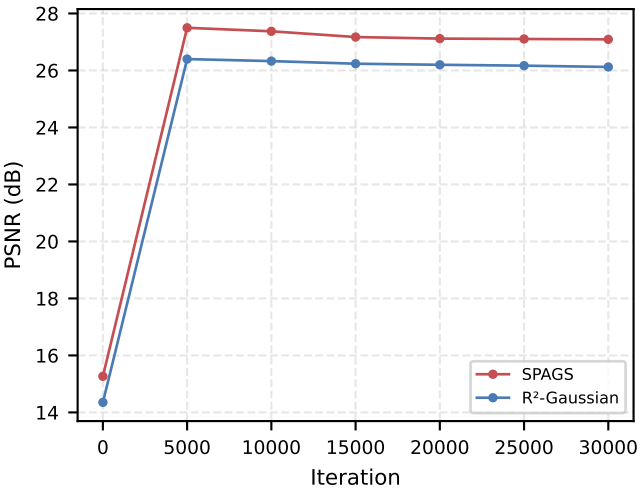
PSNR vs Iteration (Chest, 3-view)
