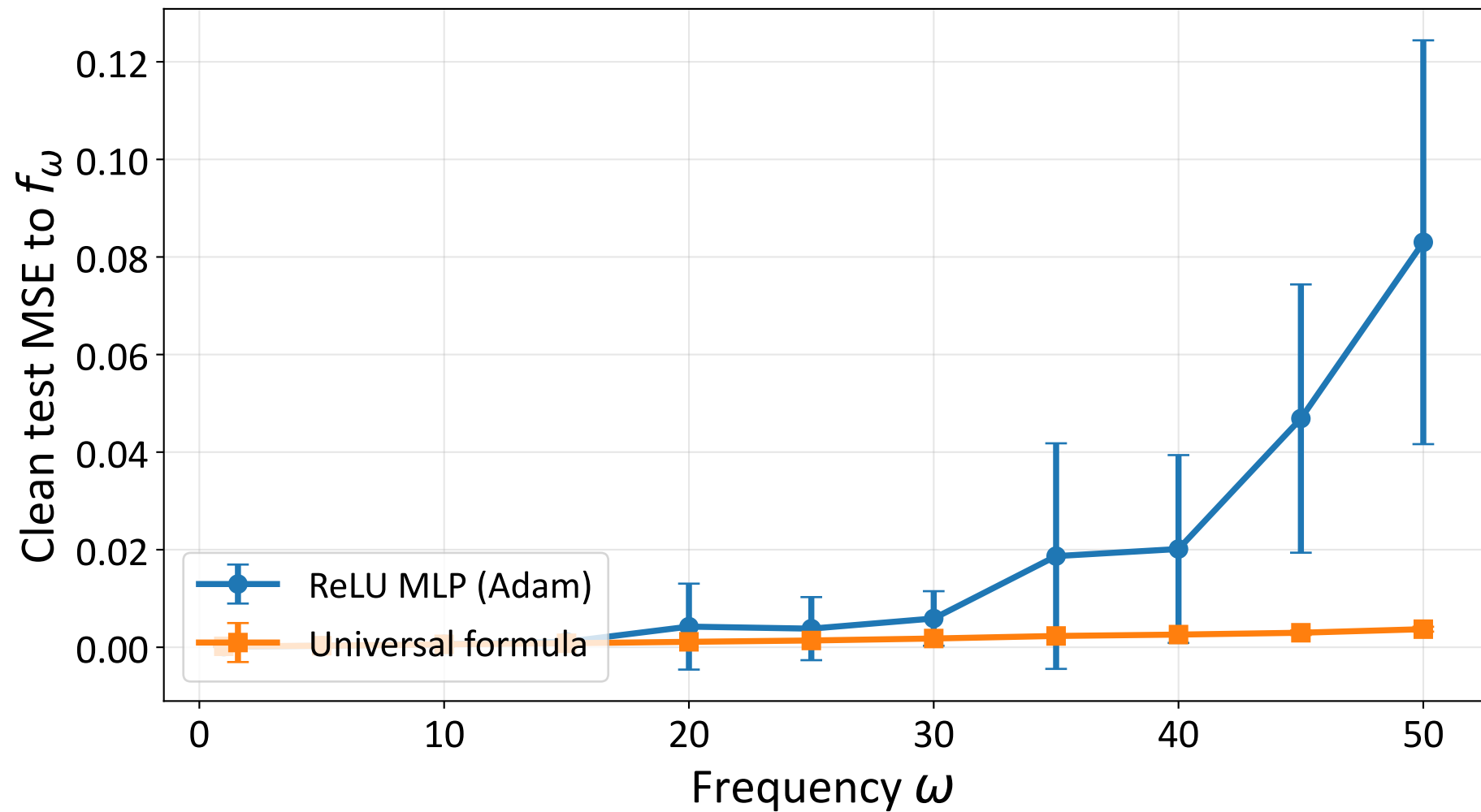
Clean recovery error versus frequency, \sigma = 0.1
