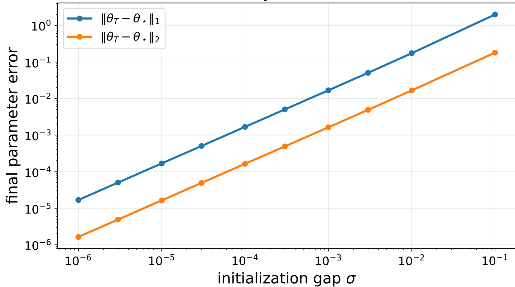
GD recovery for fixed \lambda = 1.0
