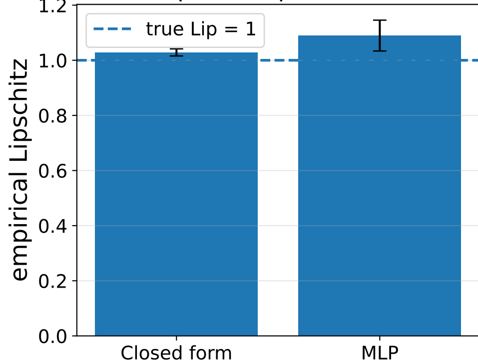
Empirical Lipschitzness
