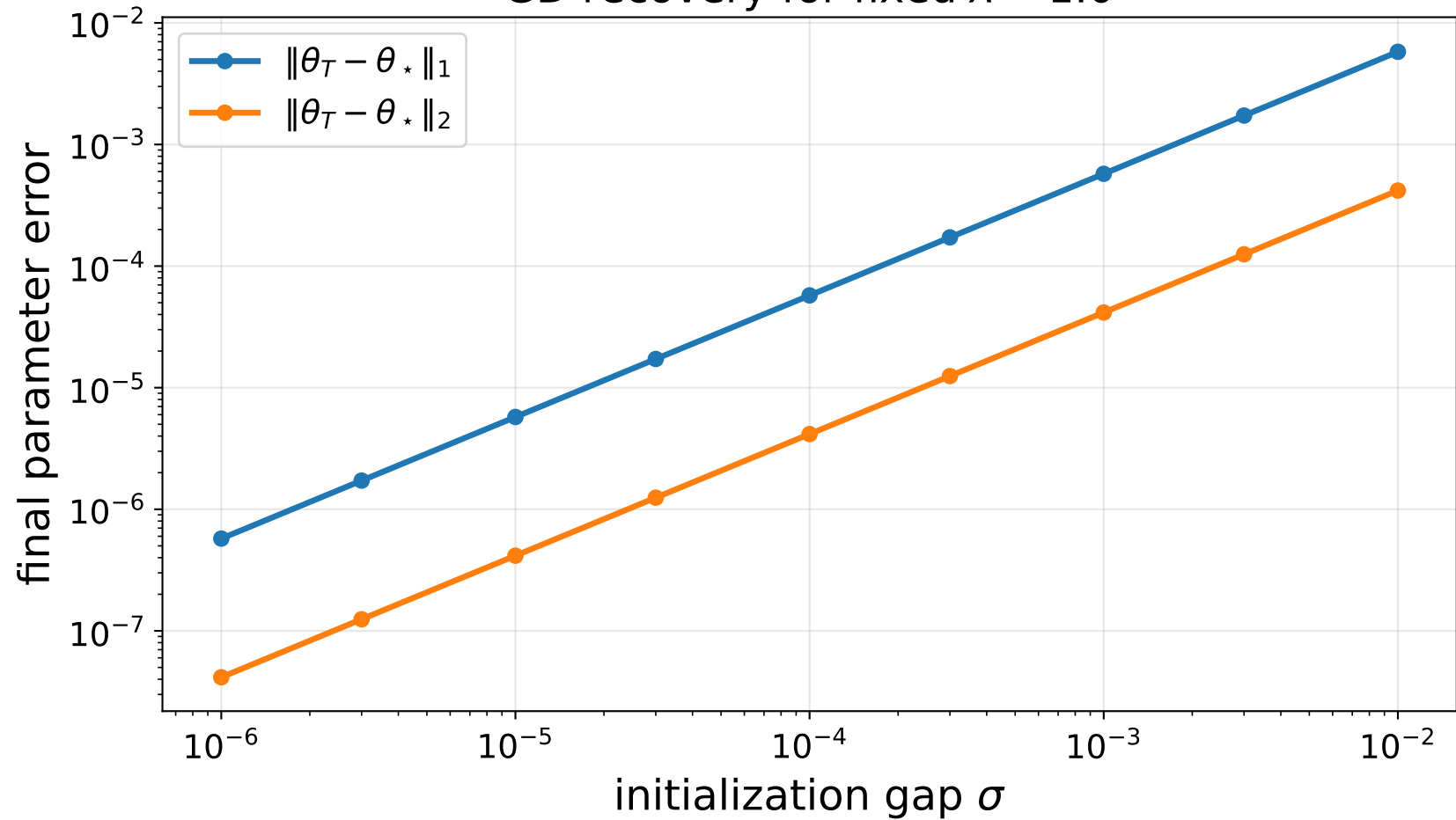
GD recovery for fixed \lambda = 1.0
