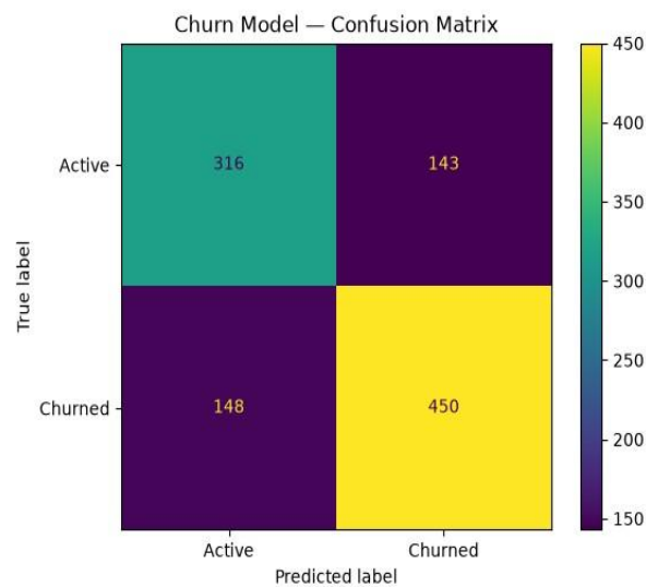
Figure: Confusion matrix at 0.5 probability threshold — 316 true negatives, 143 false positives, 148 false negatives, 450 true positives.
