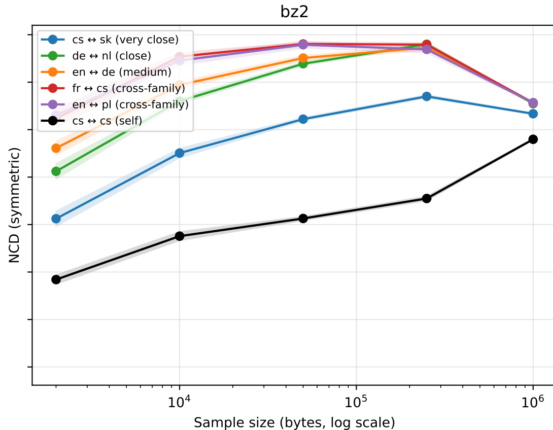
Symmetric NCD vs. sample size by compressor
