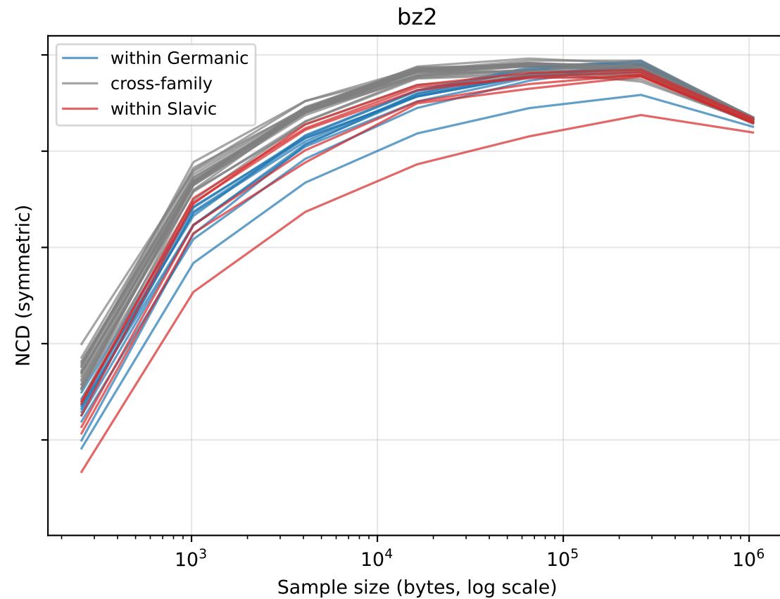
Symmetric NCD vs. sample size — all pairs
