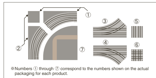
40-102-E UNITRAM E Series Intersection Road Plate $22.00
