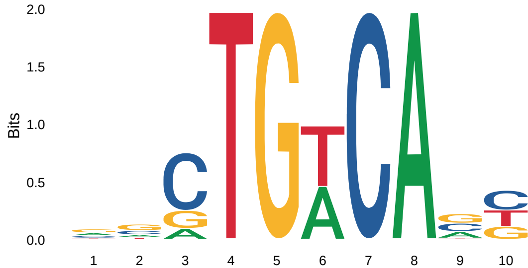
Meis1(Homeobox)/MastCells-Meis1-ChIP-Seq(GSE48085)/Homer
