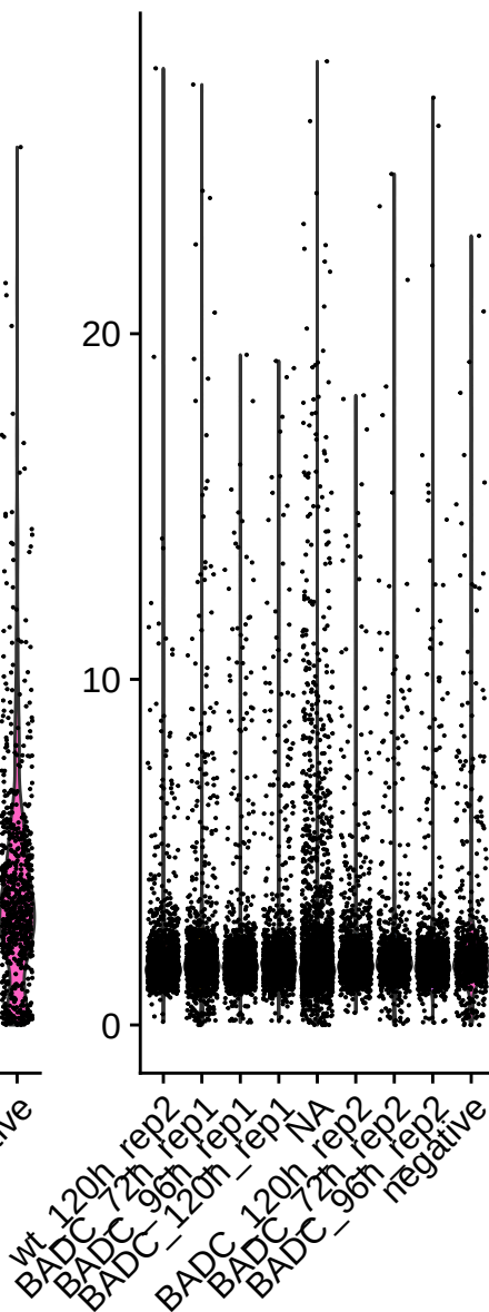
percent.mt
