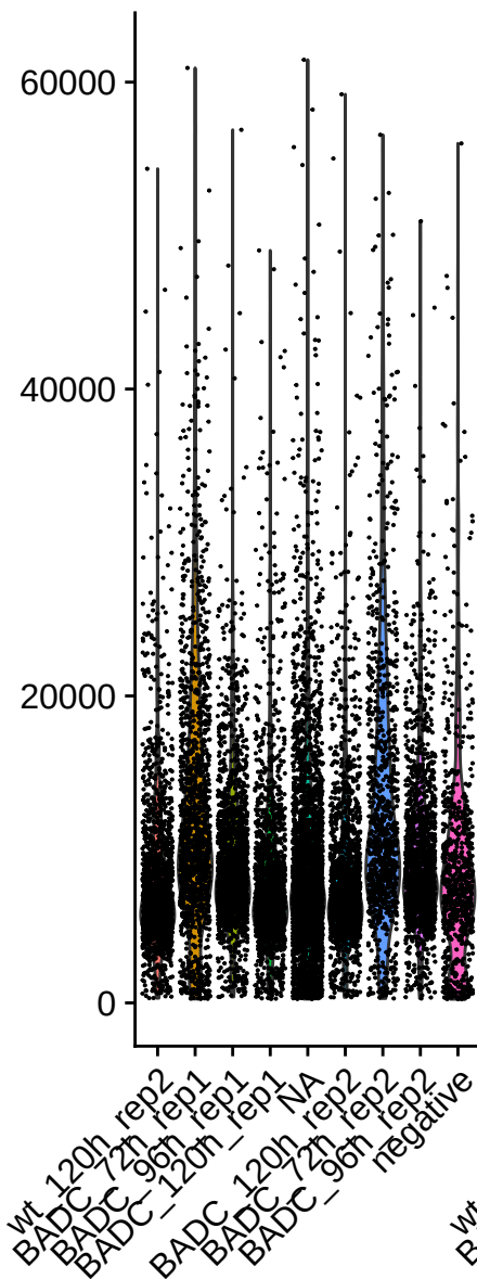
nCount_RNA
