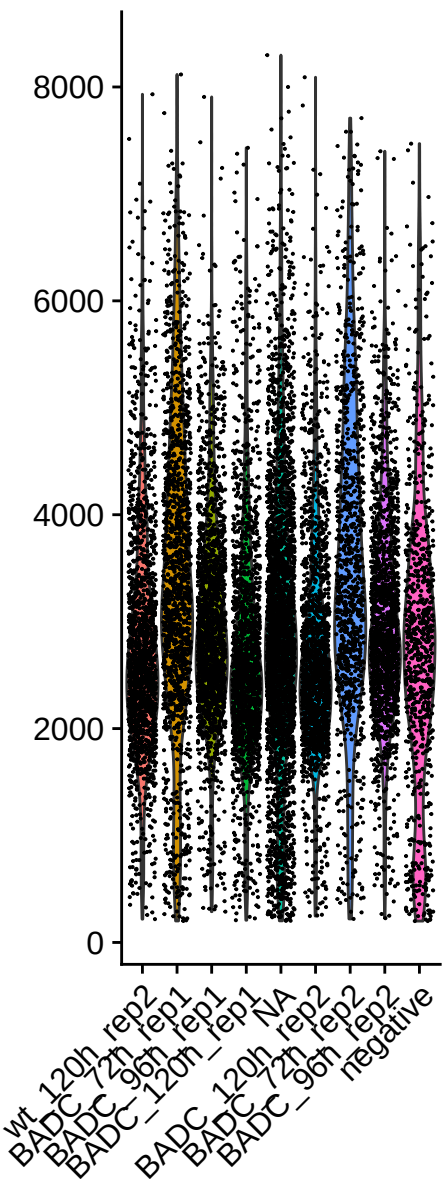
nFeature_RNA
