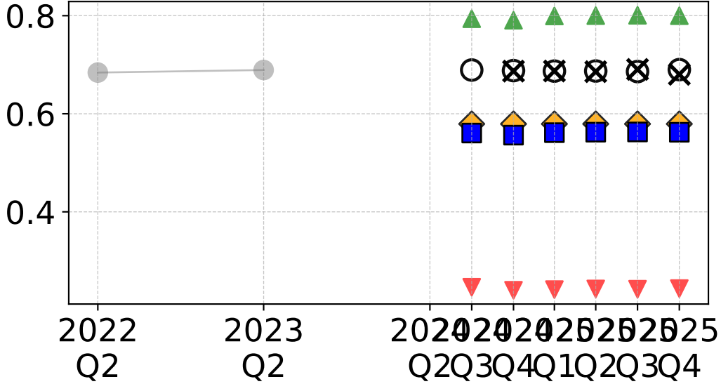
theta_DSO
