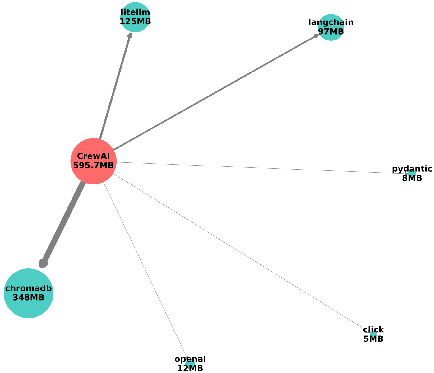
CrewAI Dependencies (595.7MB)
