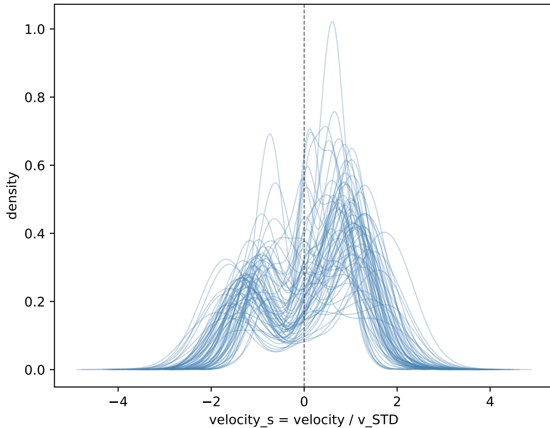
Per-animal velocity KDE (n=68 recordings)
