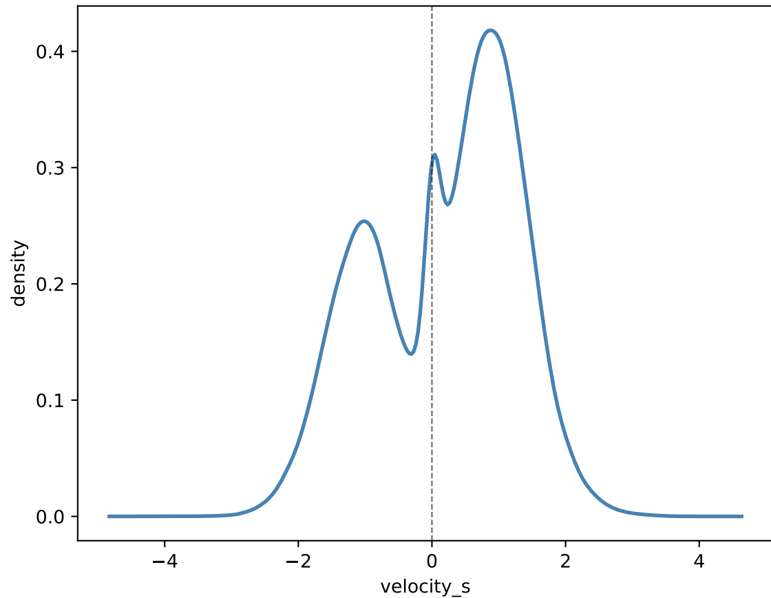
Pooled velocity KDE (n=109,052 frames)
