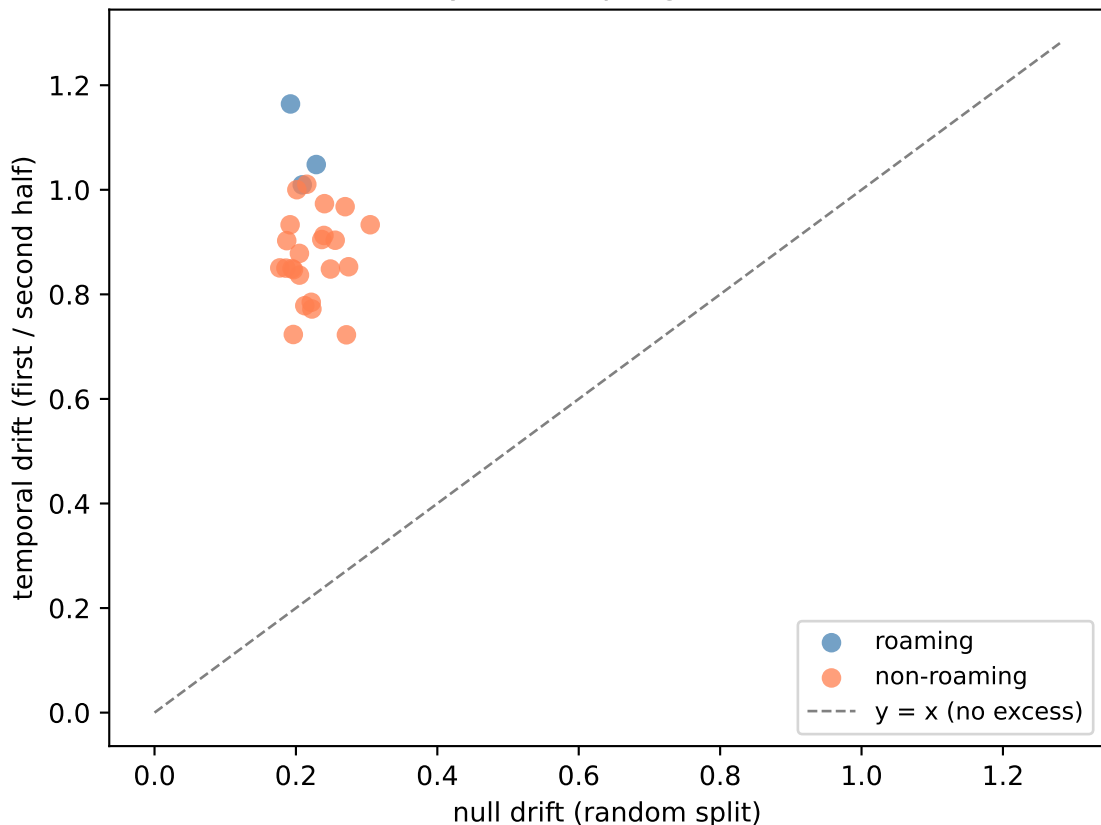
Temporal vs null-split covariance drift Points near y=x : sampling noise dominates
