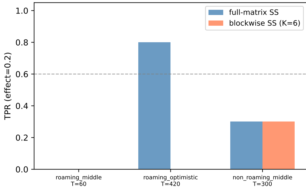
Blockwise vs full-matrix (K=6 blocks)
