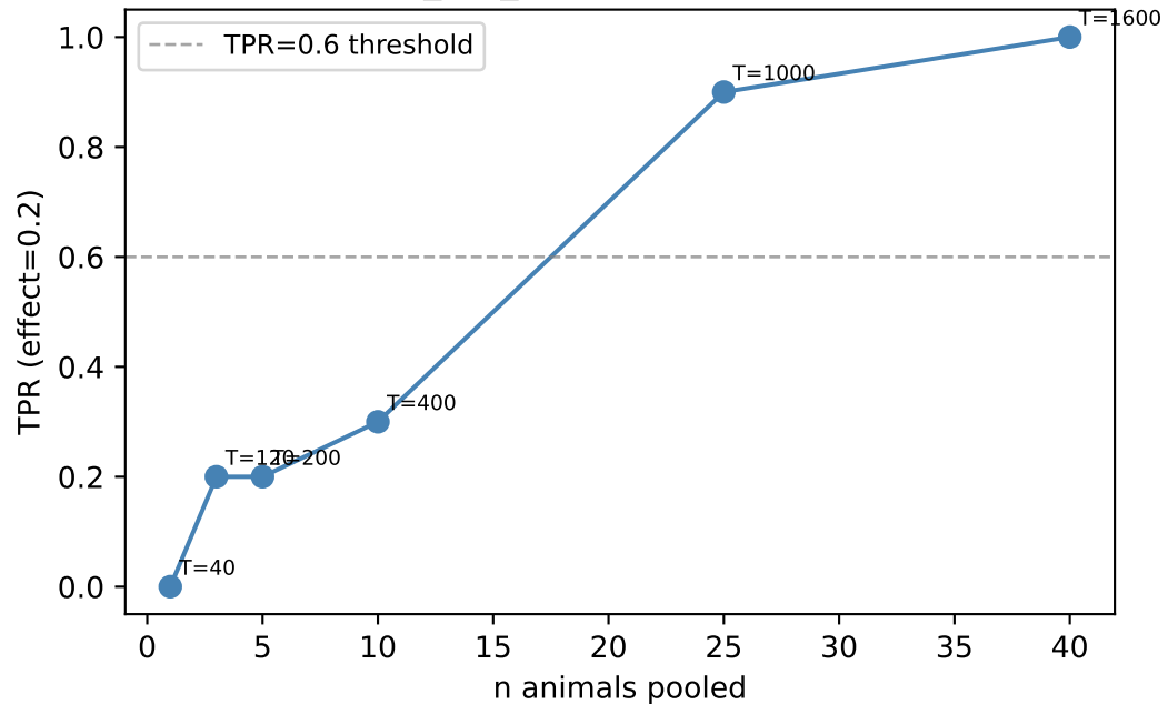
Pooled multi-animal recovery ( T_{\text{per\_animal}}=40 , N=61 )
