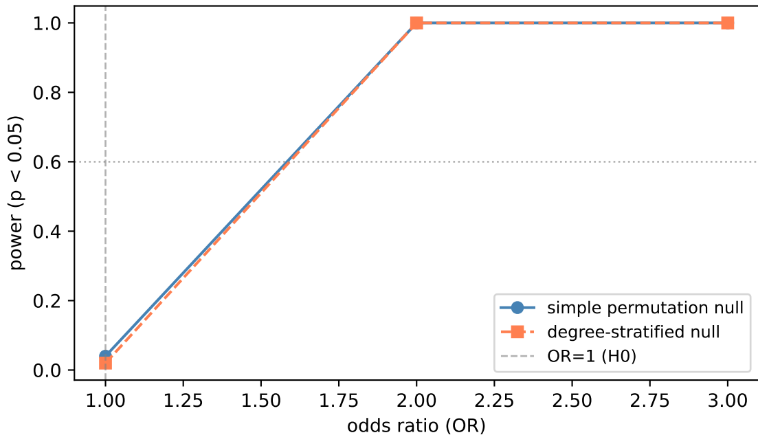
Null model calibration comparison (AUROC power under simple vs degree-stratified null)
