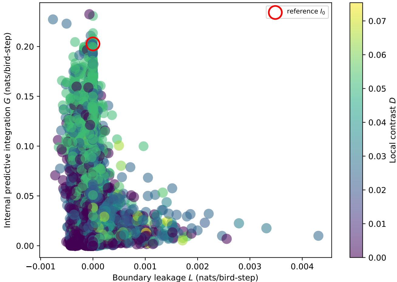
Figure 6.6-1: Collective landscape, seed 2, no_control (5000 candidate k=20 interiors; size = coherence C )
