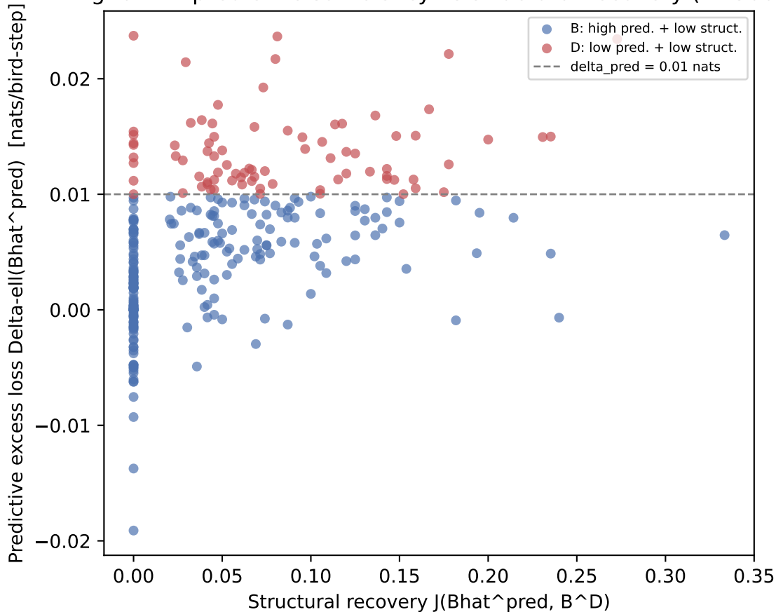
Fig. 6.7-1: predictive sufficiency vs structural recovery (n=300)
