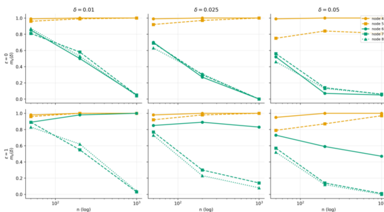
Figure 6 — Graded membership as statistical selection stability (fixed-interior problem)
