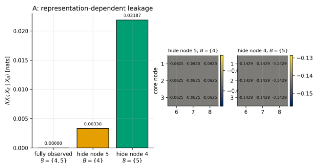
Figure 4 — Observer/representation dependence of the inferred blanket
