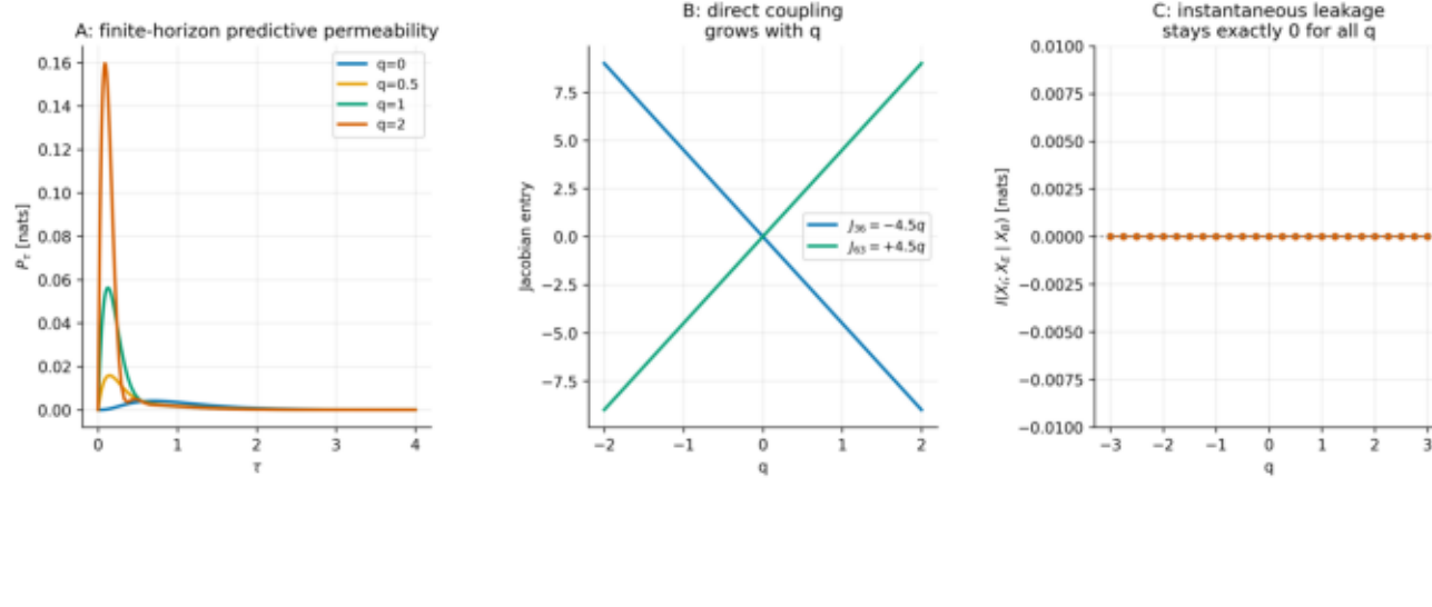
Figure 8 — Static blanket vs. finite-time dynamics are distinct objects
