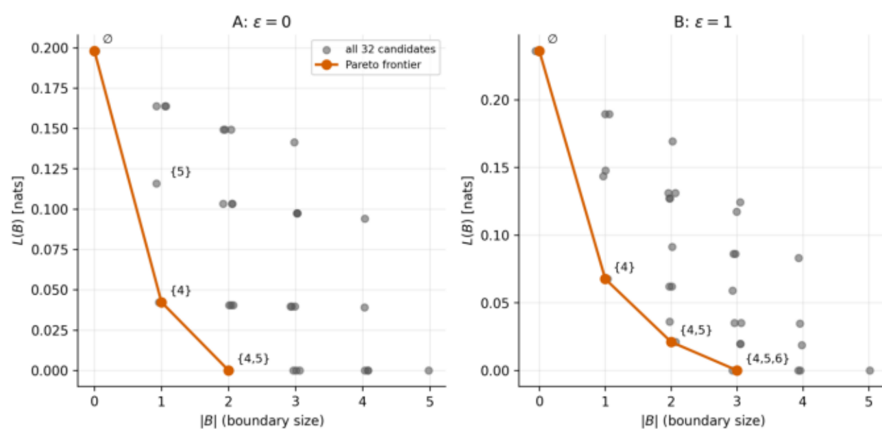
Figure 2 — Boundary complexity vs. leakage, fixed I = \{1, 2, 3\}
