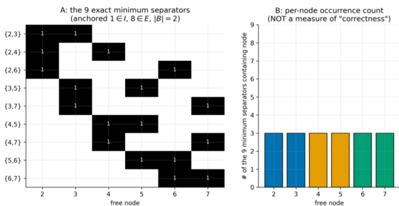
Figure 7 — Structural ambiguity is not sampling uncertainty (infinite-data result)
