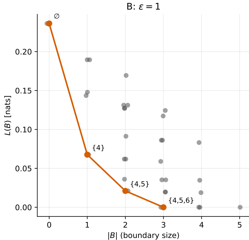
Figure 2 — Boundary complexity vs. leakage, fixed l = \{1, 2, 3\}
